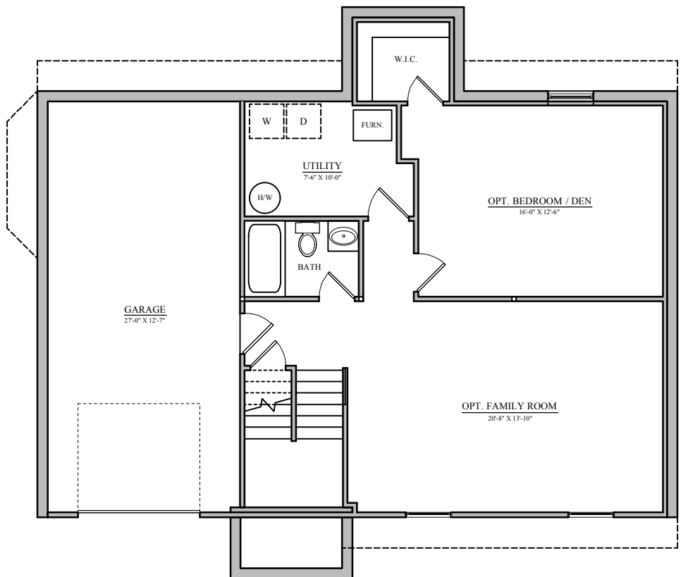
FINISHED BASEMENT PLAN DERRFIELD
